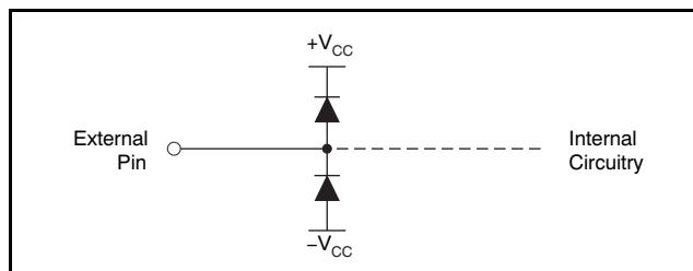
Figure 63. Internal ESD Protection
