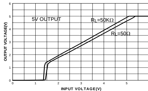
Figure 2. Dropout Characteristics
