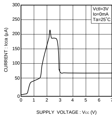
Fig.3 I_{cca} vs. V_{cc}
