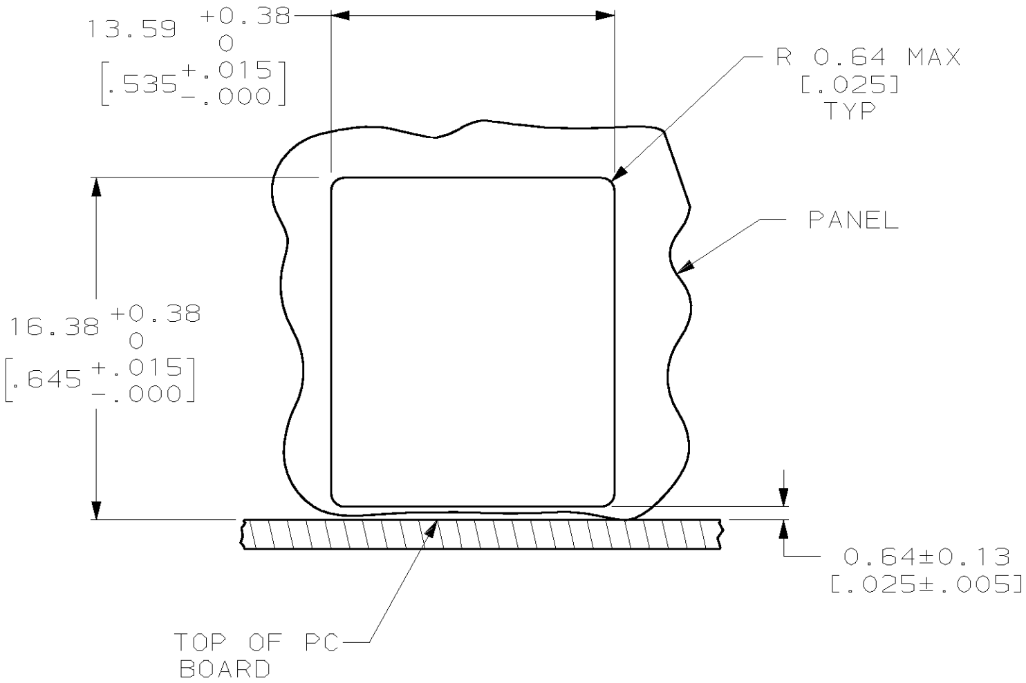
PANEL CUTOUT
