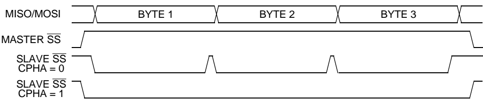
Figure 14-12. CPHA/ \overline{SS} Timing
