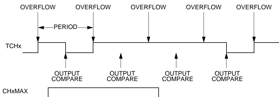
Figure 11-11. CHxMAX Latency
