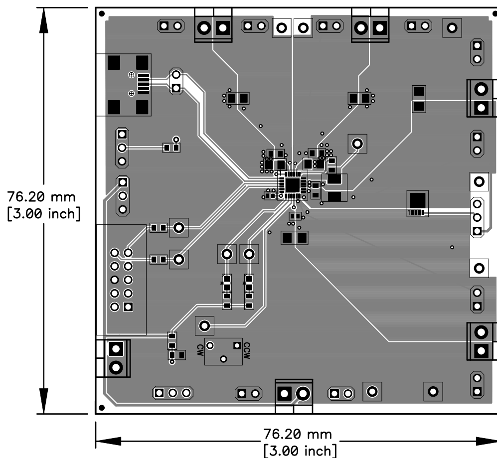
Figure 7. Top Layer
