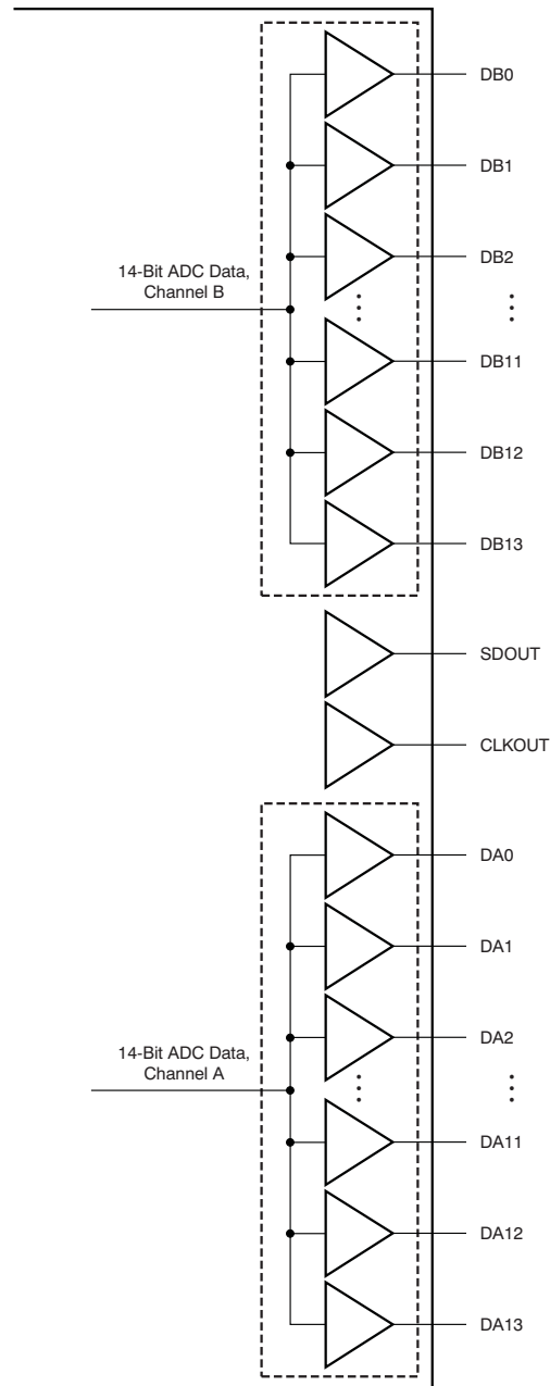
Figure 170. CMOS Outputs
