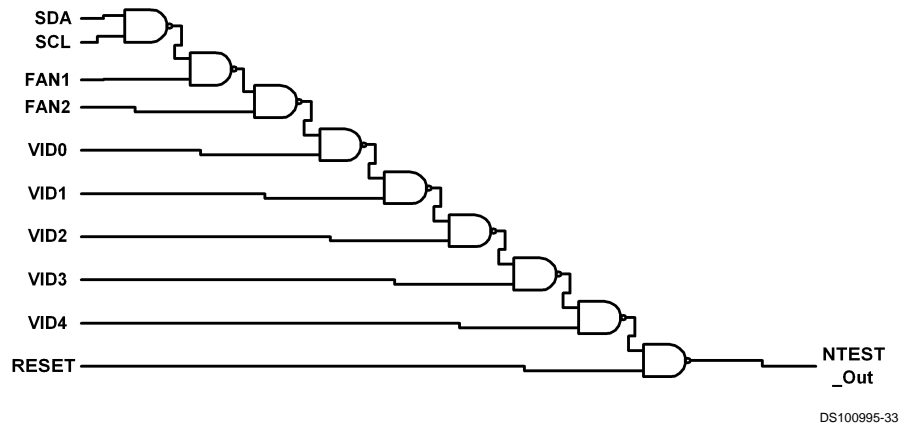
FIGURE 12. NAND Tree Test Structure
