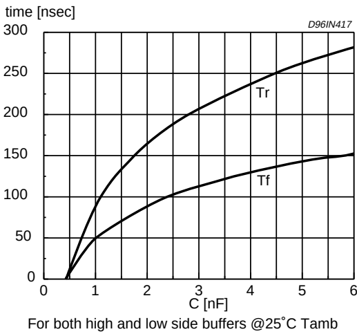
Figure 9. Typical Rise and Fall Times vs. Load Capacitance
