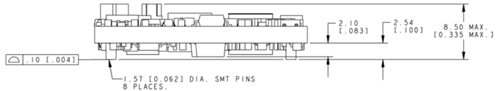
Side View
