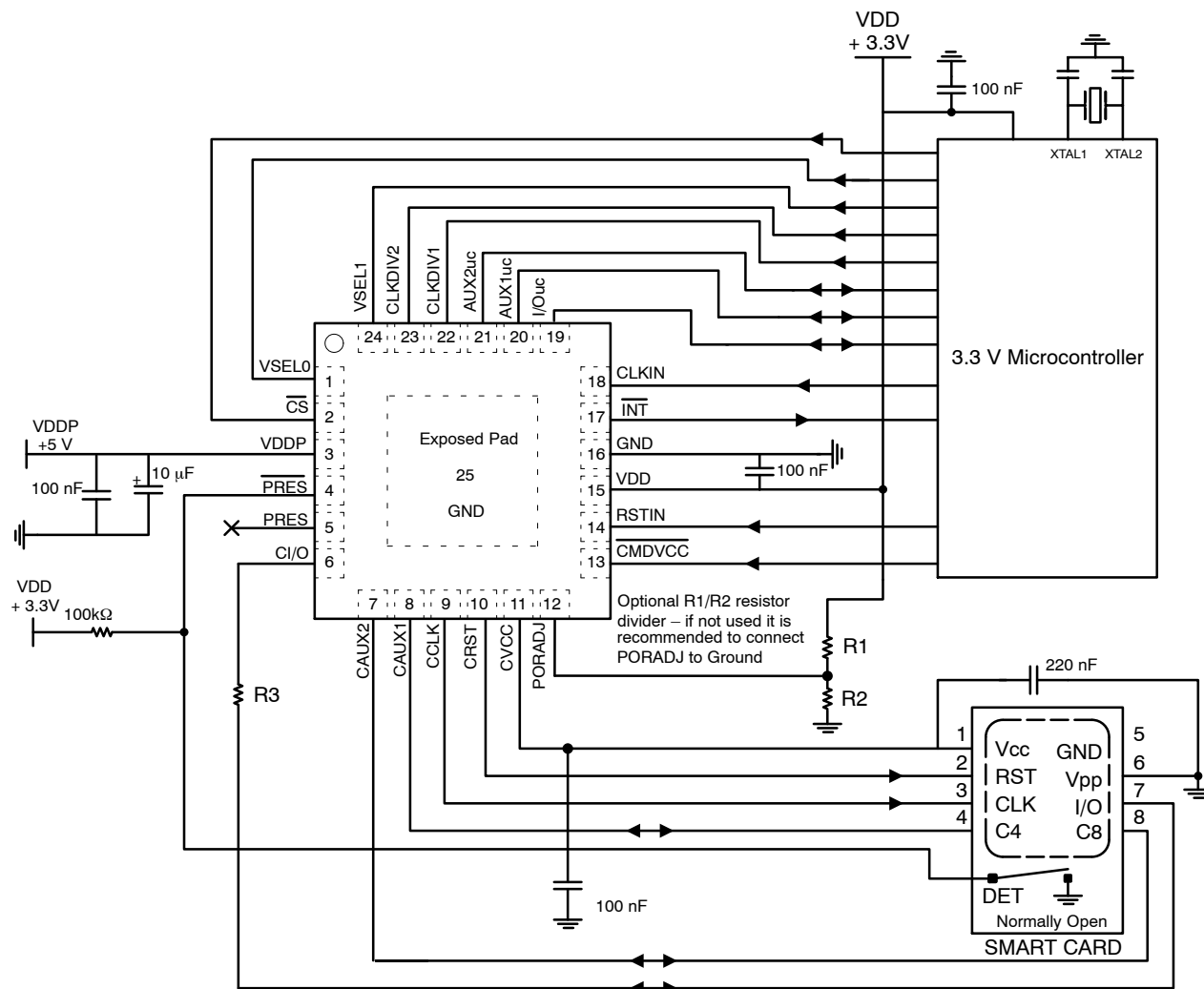
Figure 8. Application Schematic
