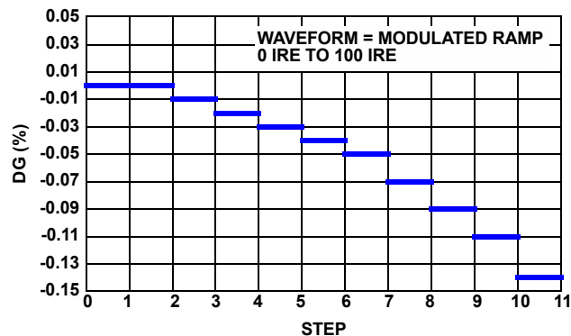
FIGURE 12. DIFFERENTIAL GAIN
