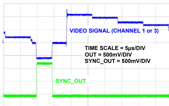
FIGURE 20. SYNC_OUT SIGNAL
