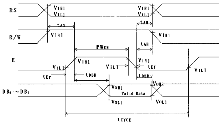
fig. 2 The timing characteristics of the bus read operating sequence. (Read from NJU6420B to MPU)
