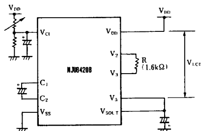
(b) 1/5 Bias (1/16 Duty) (Internal Voltage Doubler Using Example)
