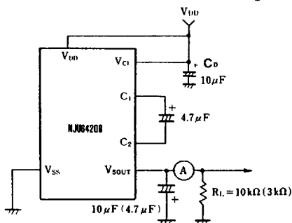
Note 9) Voltage Doubler Characteristics Measuring Circuit.
