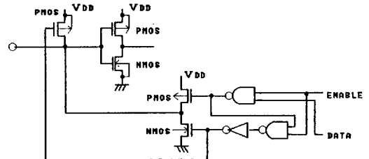
Input/Output Terminal Structure
