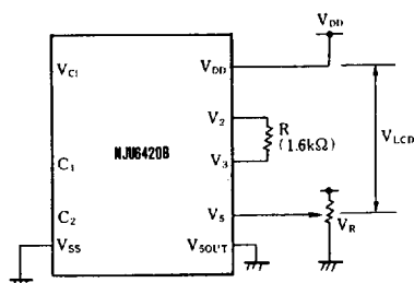
(a) 1/5 Bias (1/16 Duty) (Internal Voltage Doubler No-use Example)
