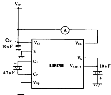
Note 9) Voltage Doubler Characteristics Measuring Circuit.
