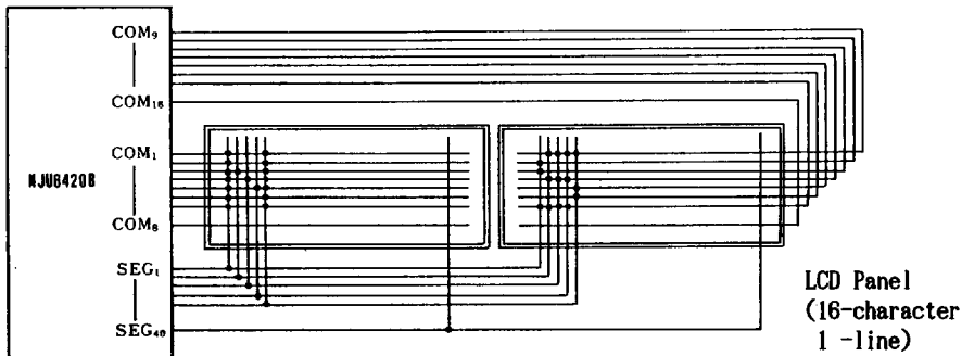
(b) 5 x 7 dots, 16-character 1-line display example (1/5 Bias, 1/16 Duty)
