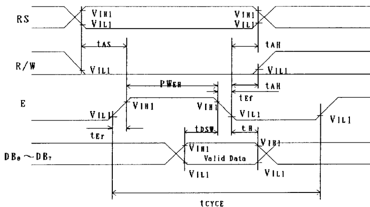
fig. 1 The timing characteristics of the bus write operating sequence. (Write from MPU to NJU6420B)
