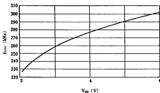
Note 10) Supply Voltage vs Oscillation Frequency
