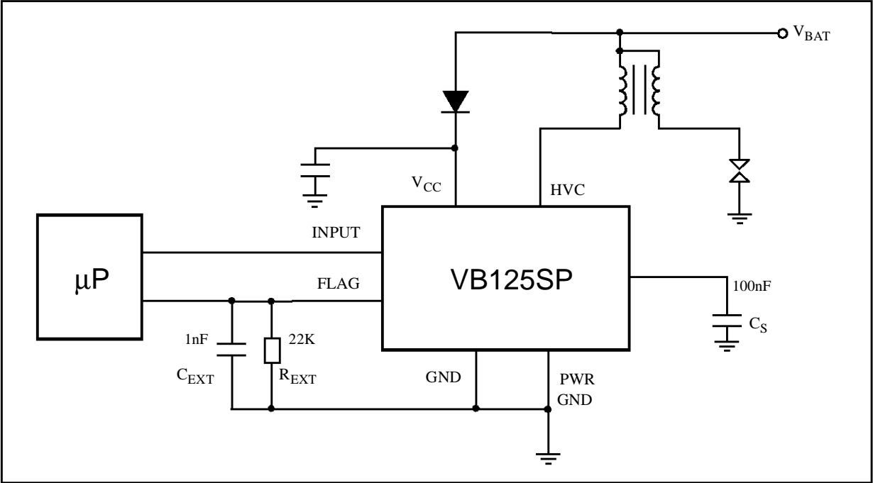
FIGURE 7: Application Circuit
