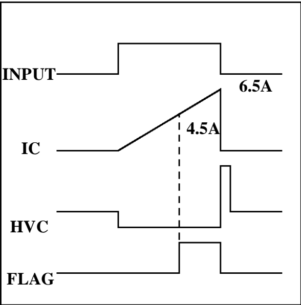
FIGURE 5: Waveforms
