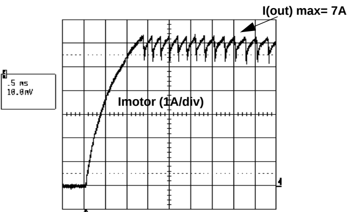
Figure 14. Current Limitation
