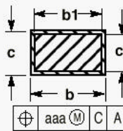
SECTION W-W
