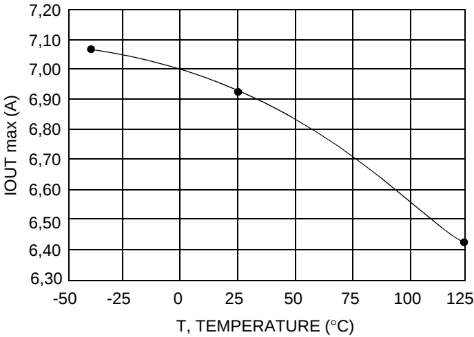
Figure 14. Current Limitation
