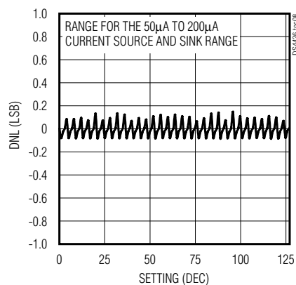
DIFFERENTIAL LINEARITY
