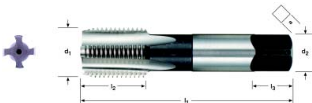
G Series (BSPF) Taps, Straight Flute
