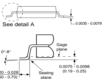
DETAIL A Typ. Scale: 40X
