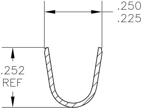
SECT C-C
