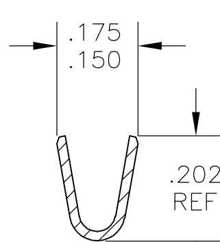
SECT B-B
