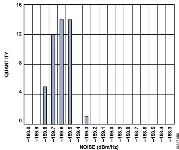
Figure 23. 20 MHz Offset Noise Floor Distribution at f_{LO} = 3500 MHz (I/Q Amplitude = 0 mV p-p with 500 mV dc Bias)
