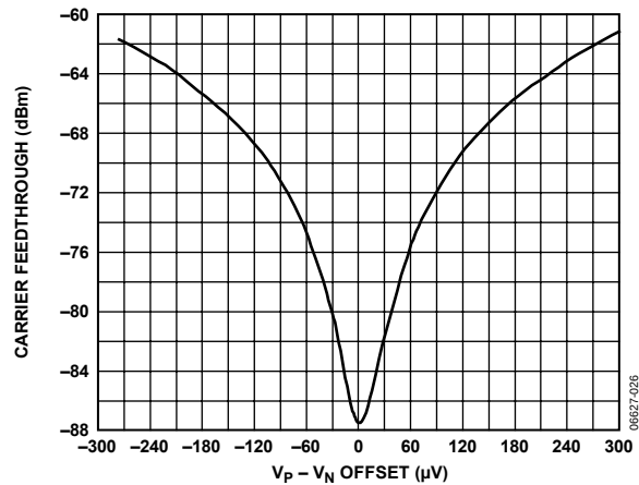
Figure 26. Carrier Feedthrough vs. DC Offset Voltage at 3500 MHz
