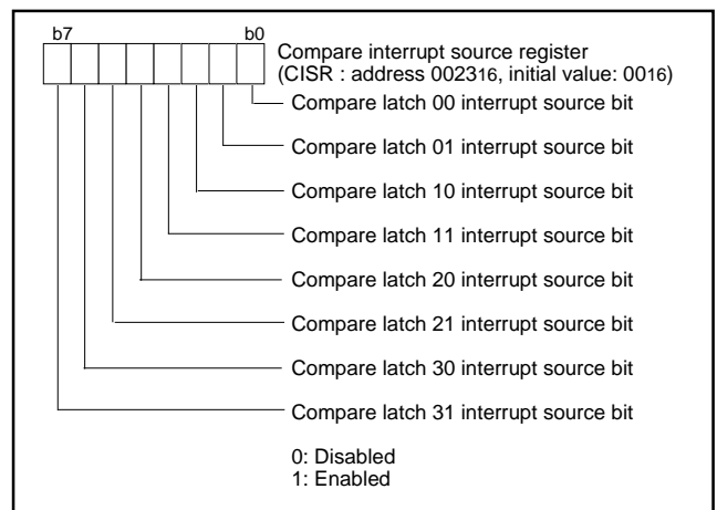
Fig. 31 Structure of compare interrupt source register
