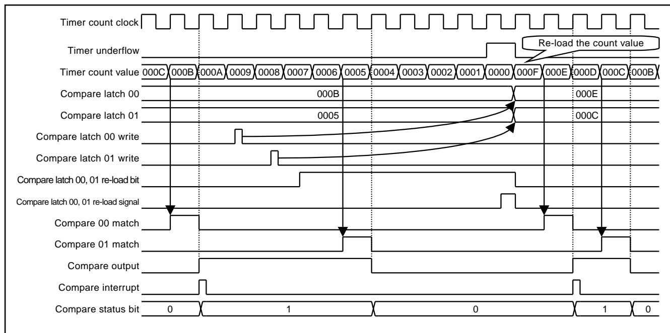
Fig. 36 Output compare mode (compare register write timing)
