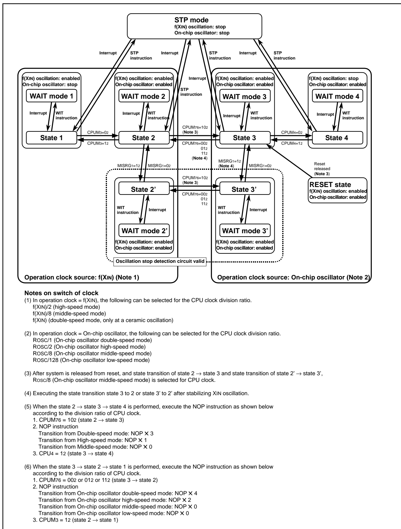
Fig. 75 State transition
