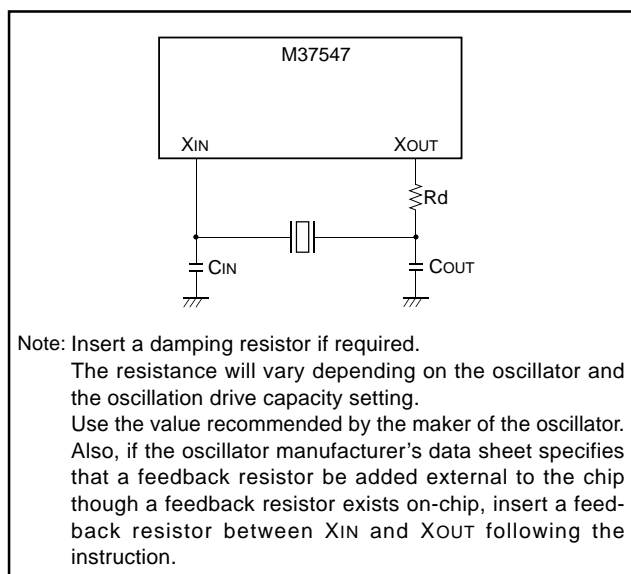
Fig. 68 External circuit of ceramic resonator
