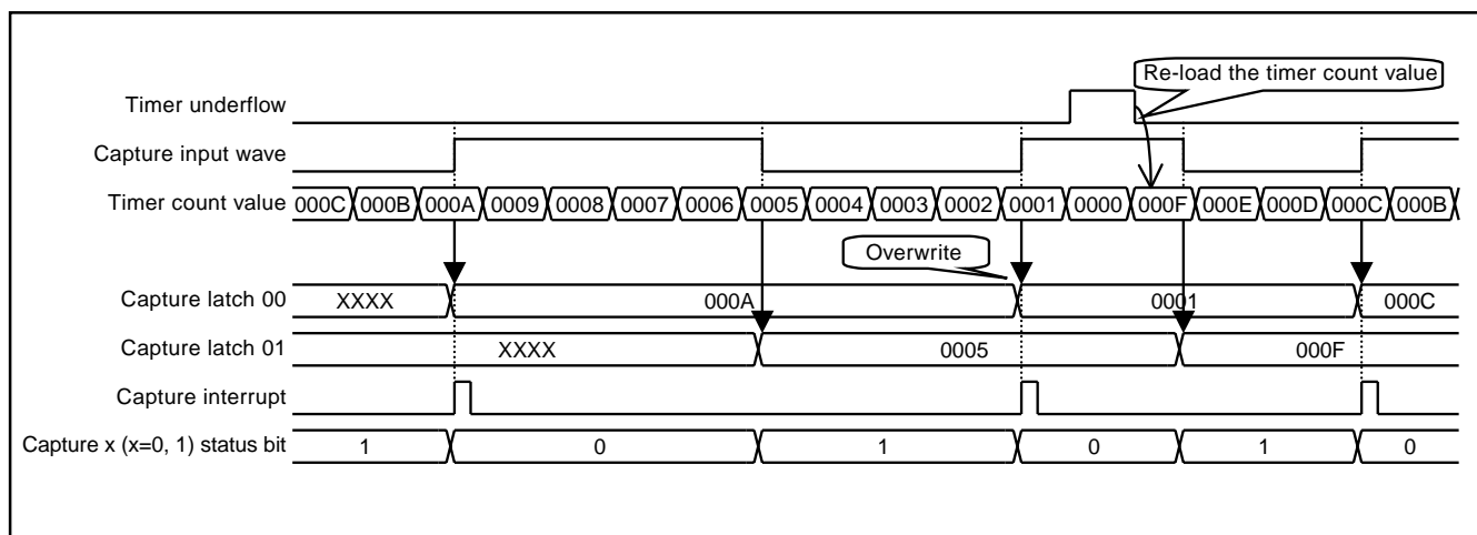
Fig. 43 Capture interrupt edge selection = "rising edge"
