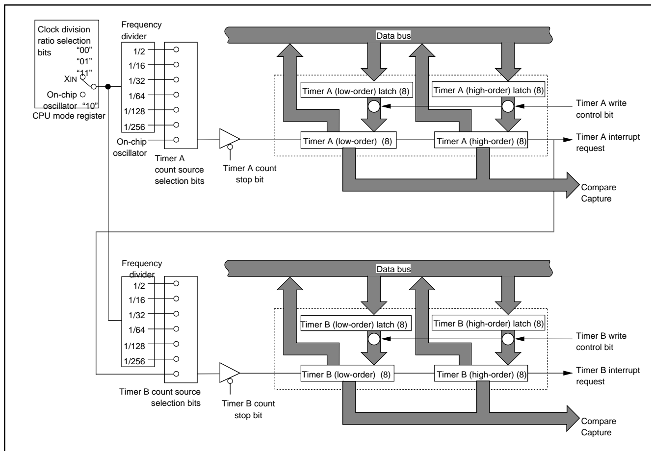
Fig. 24 Block diagram of timer A and timer B
