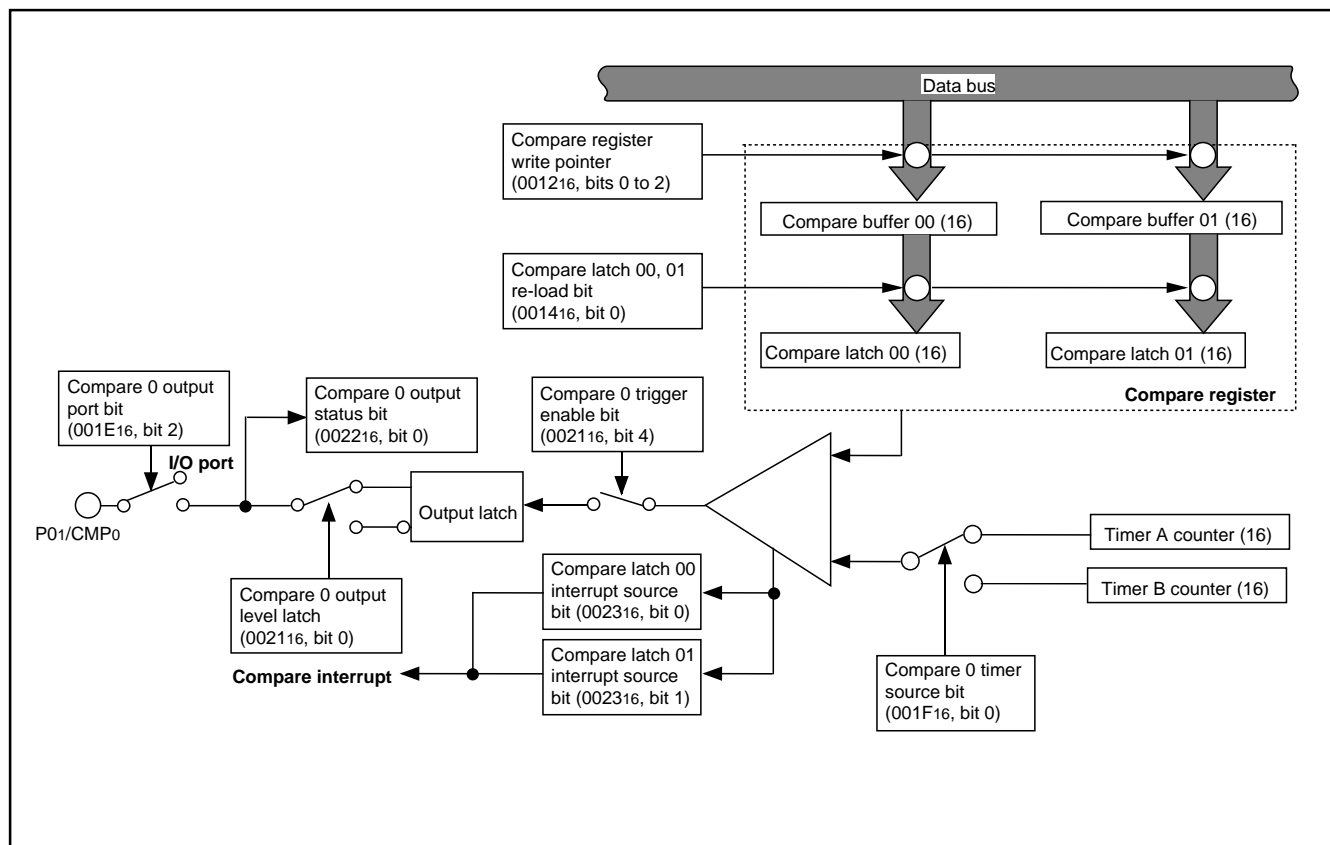
Fig. 33 Block diagram of compare channel 0
