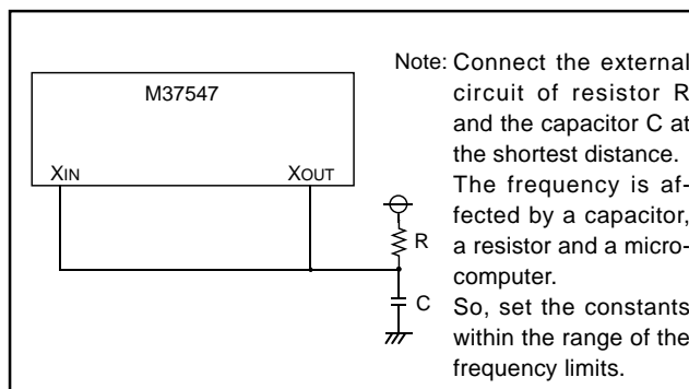
Fig. 69 External circuit of RC oscillation
