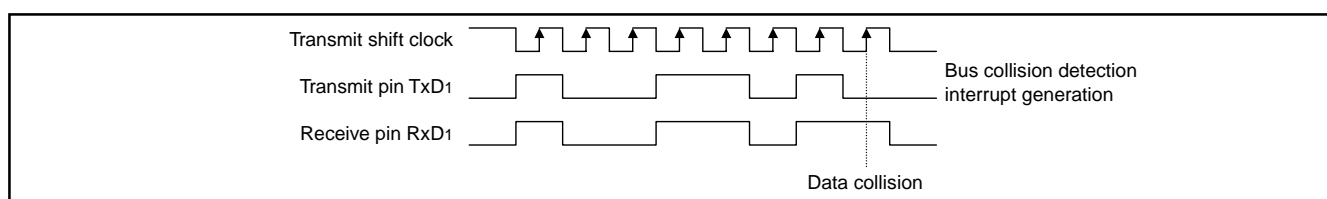
Fig. 52 Timing diagram of bus collision detection interrupt
