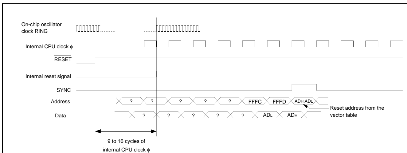
Fig. 65 Timing diagram at reset
