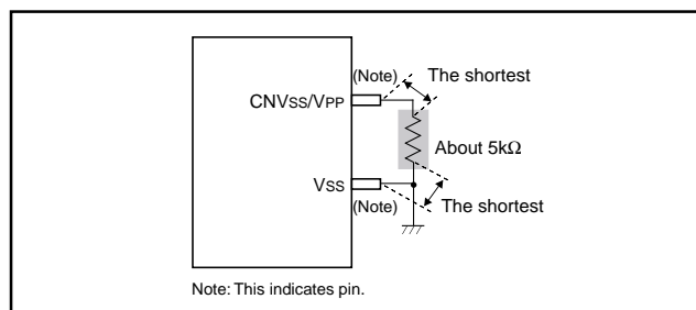
Fig. 85 Wiring for the VPP pin of the QzPROM
