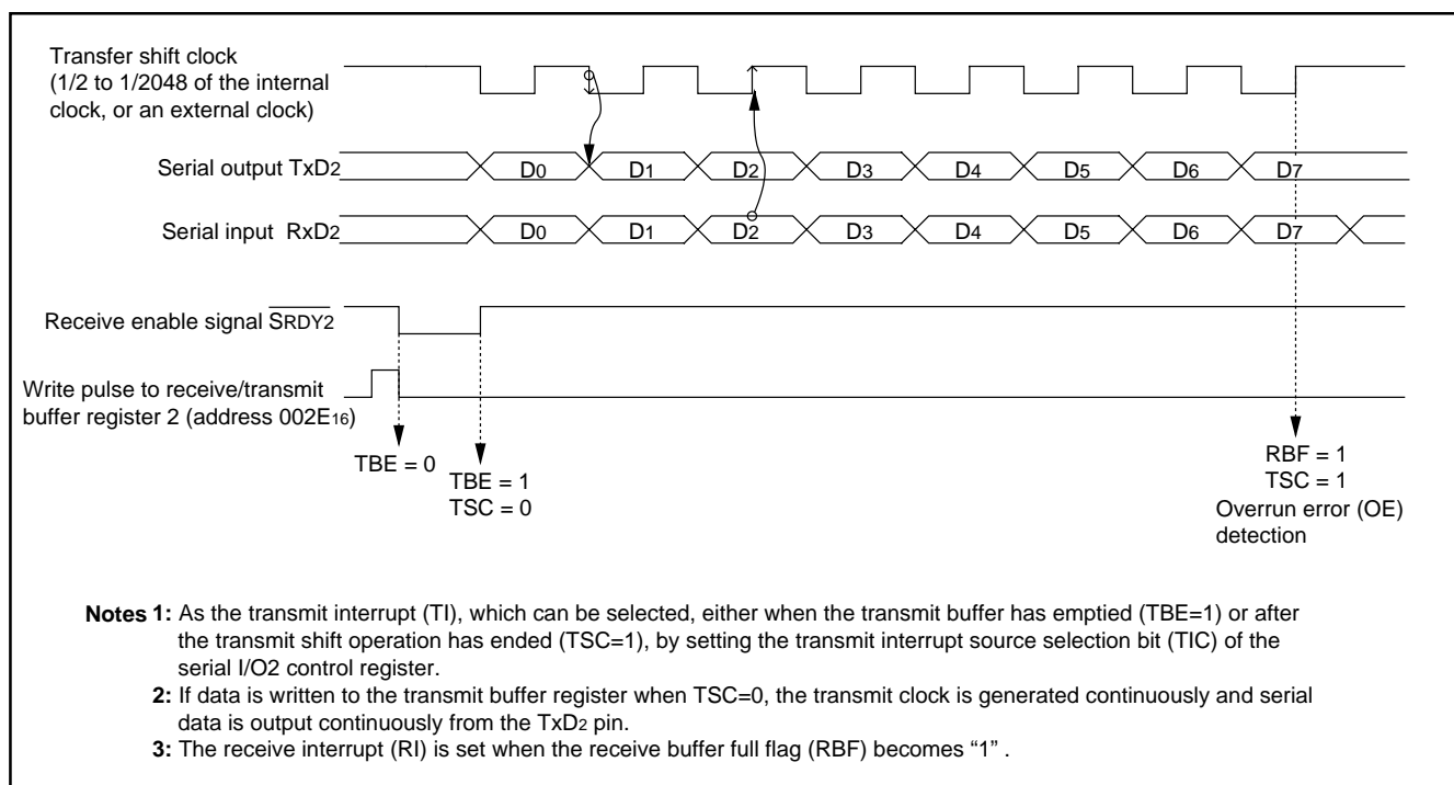
Fig. 54 Operation of clock synchronous serial I/O2 function
