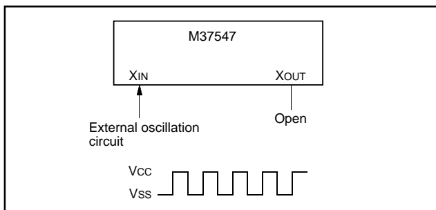
Fig. 70 External clock input circuit
