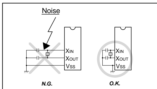
Fig. 84 Wiring for clock I/O pins
