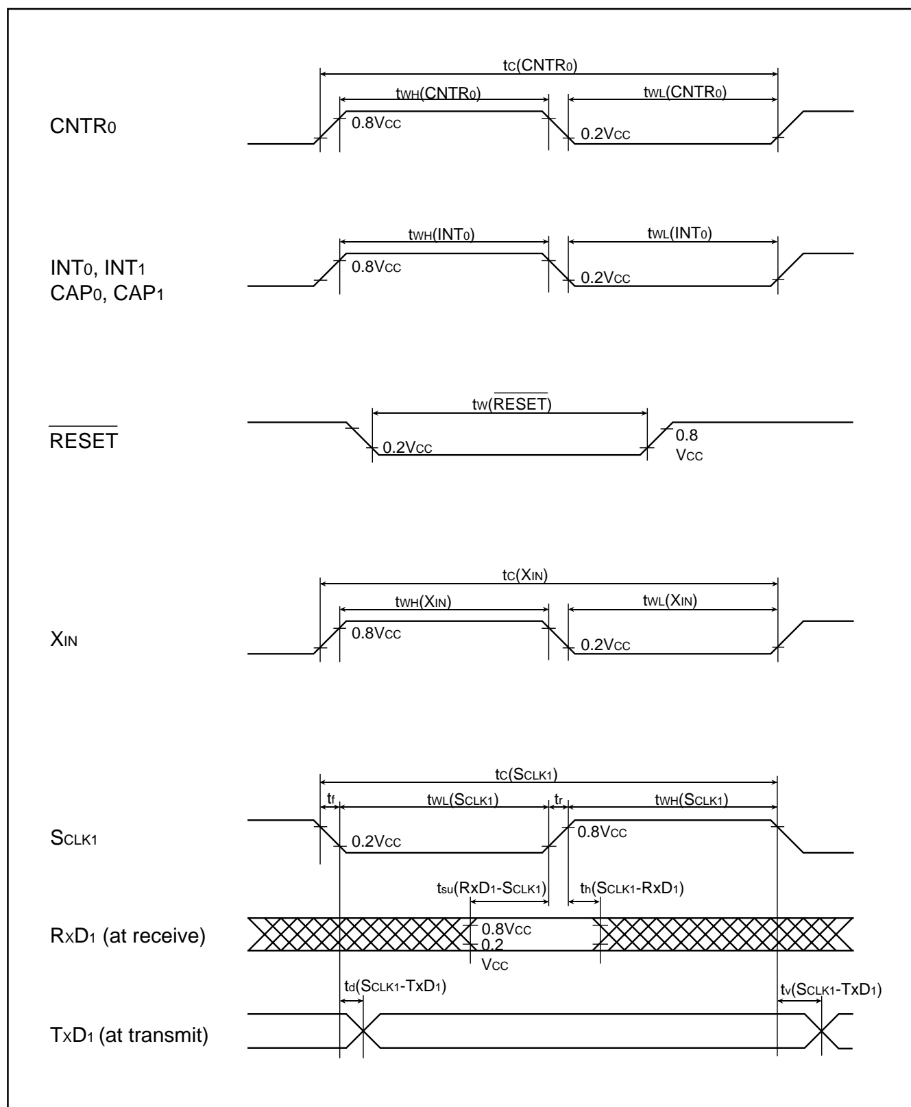
Fig. 93 Timing chart
