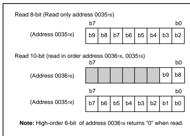
Fig. 59 Structure of A/D conversion register
