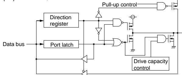
(17) Ports P3 4 , P3 5
