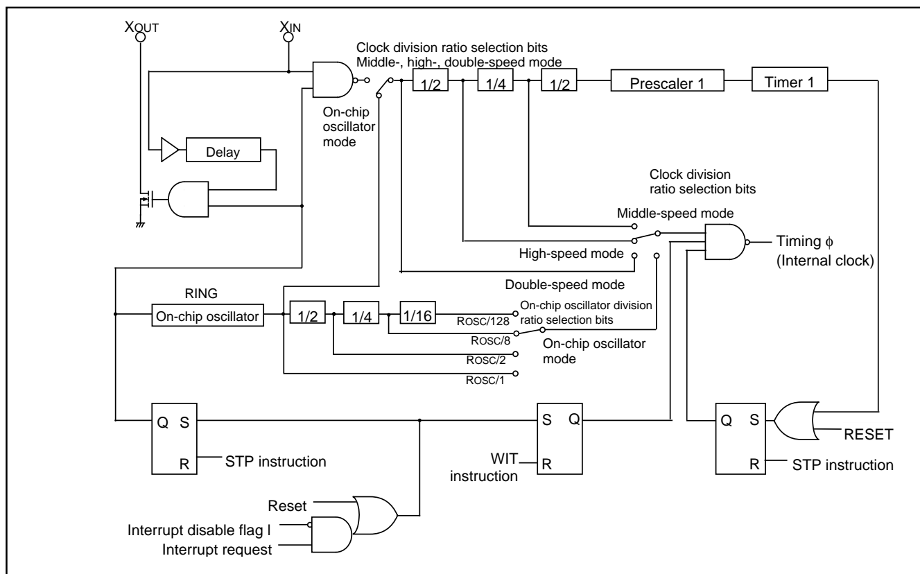
Fig. 74 Block diagram of internal clock generating circuit (for RC oscillation)
