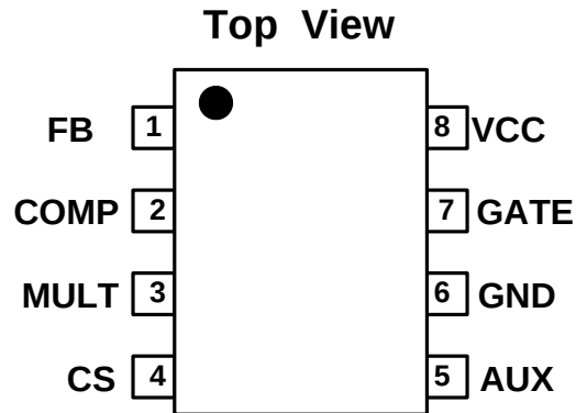
Figure 2: Pin Assignments
