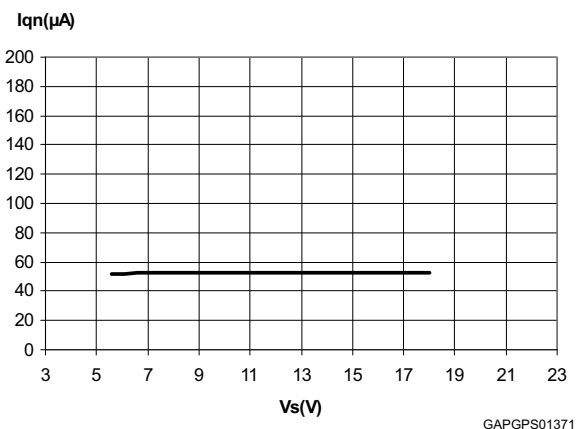
Figure 7. Current consumption vs. input voltage ( I_o = 0.1\text{ mA} )
