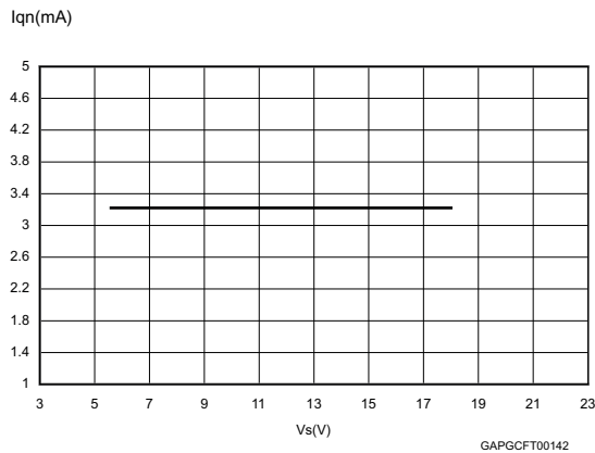
Figure 8. Current consumption vs. input voltage ( I_o = 75\text{ mA} )
