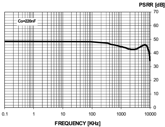
Figure 13. PSRR
