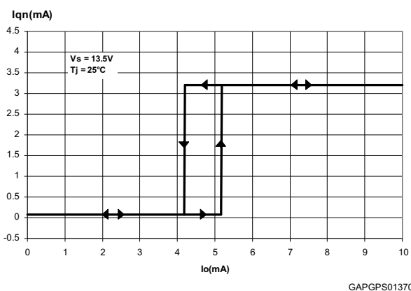
Figure 6. Current consumption vs. output current (at light load condition)
