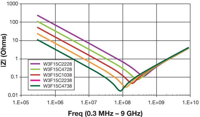
IMPEDANCE 1206 – 50V
