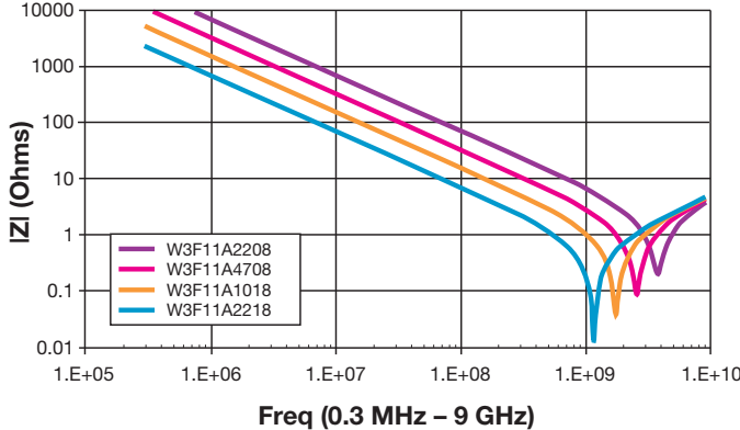
IMPEDANCE 1206 – 100V
