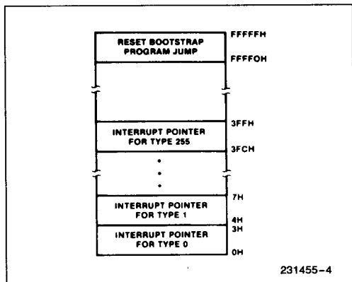
Figure 3b. Reserved Memory Locations
