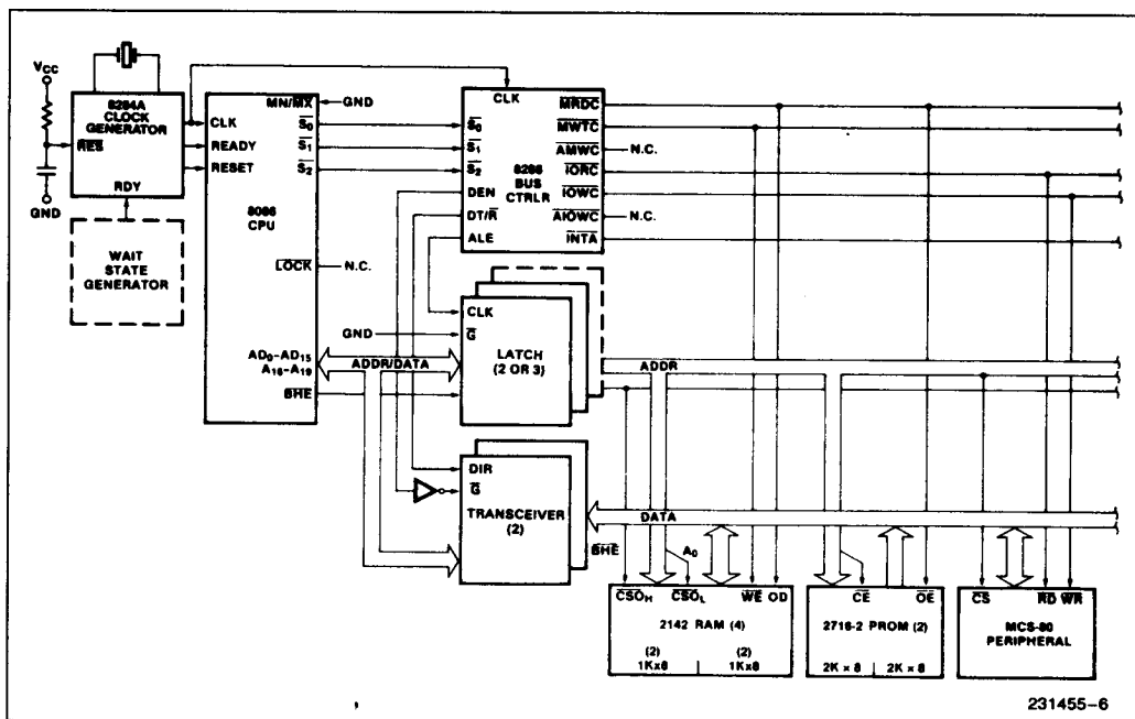
Figure 4b. Maximum Mode 8086 Typical Configuration
