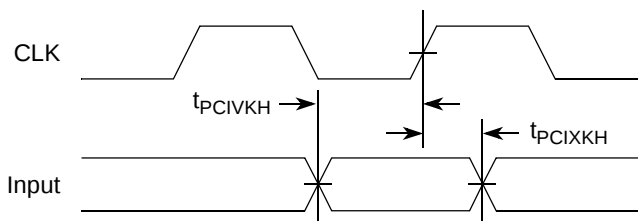
Figure 33. PCI-PCI-X Input AC Timing Measurement Conditions
