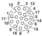
Pin assignment M12, 17-pos., female side view
