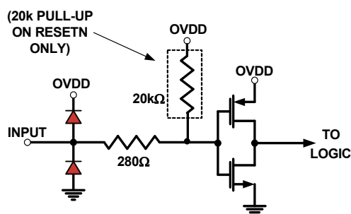
FIGURE 50. DIGITAL INPUTS
