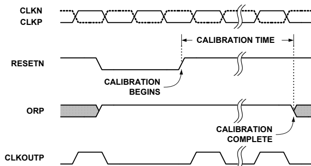
FIGURE 27. CALIBRATION TIMING
