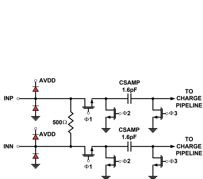
FIGURE 47. ANALOG INPUTS
