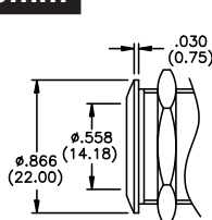
09 flat Act. & curved Bushing
