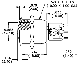
19 curved Act. & Bushing (standard)
