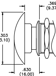
49 thd'd Act. with mushroom cap & curved bushing
