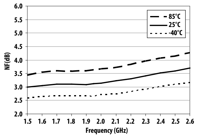
Figure 29. Noise Figure over Frequency and Temperature
