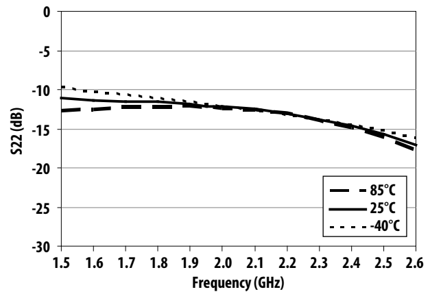
Figure 27. S22 over Frequency and Temperature
