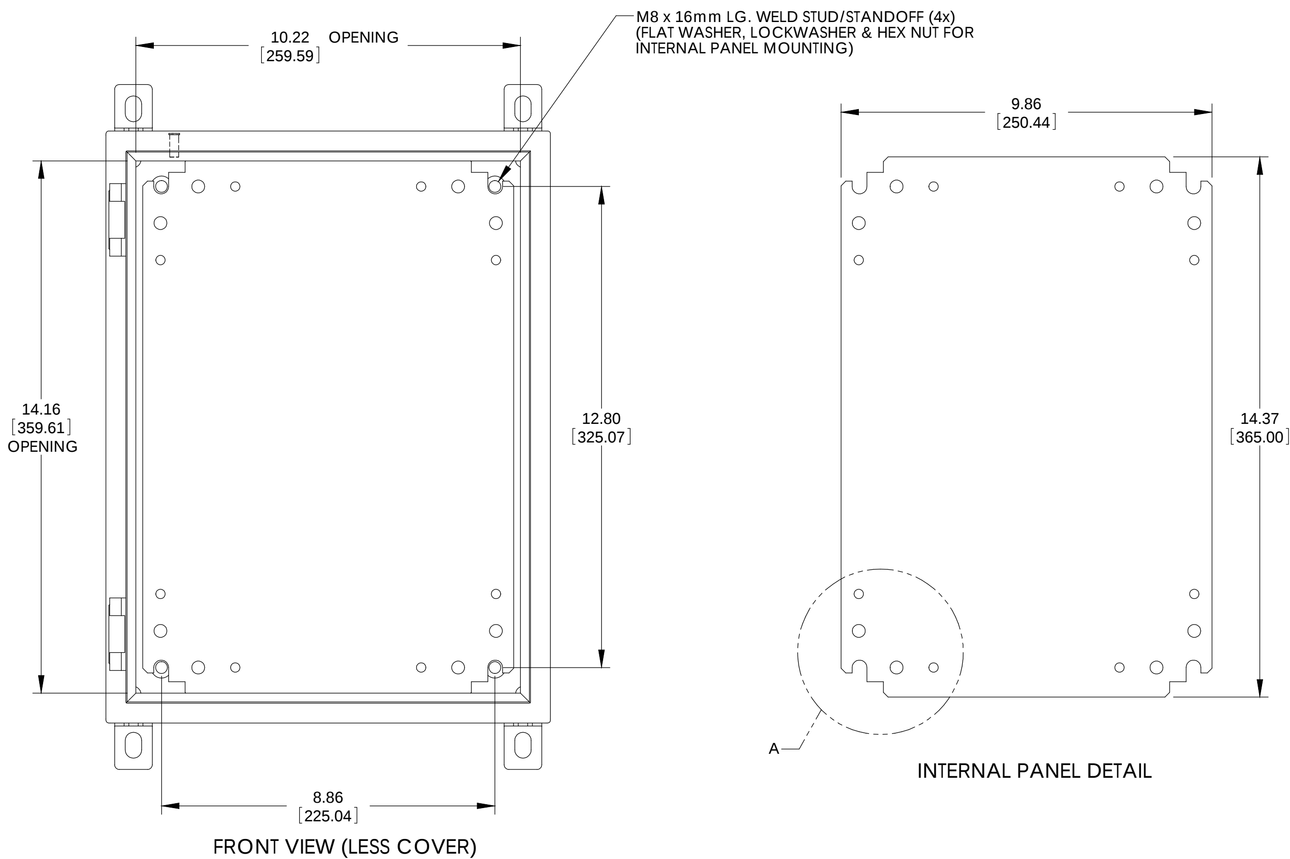
FRONT VIEW (LESS COVER)
