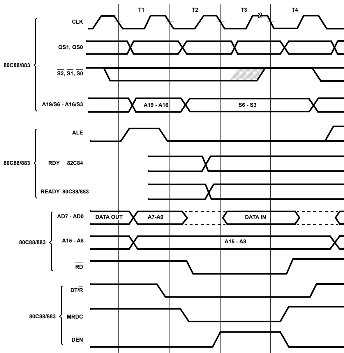
FIGURE 9. MEDIUM COMPLEXITY SYSTEM TIMING
