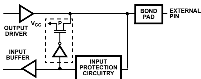
FIGURE 7. BUS HOLD CIRCUITRY PINS 26-32 AND 34
