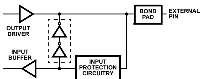
FIGURE 6. BUS HOLD CIRCUITRY PINS 2-16 AND 35-39
