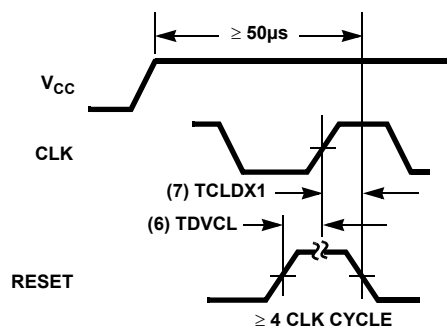
FIGURE 18. RESET TIMING
