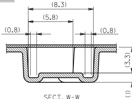
SECT. W-W
