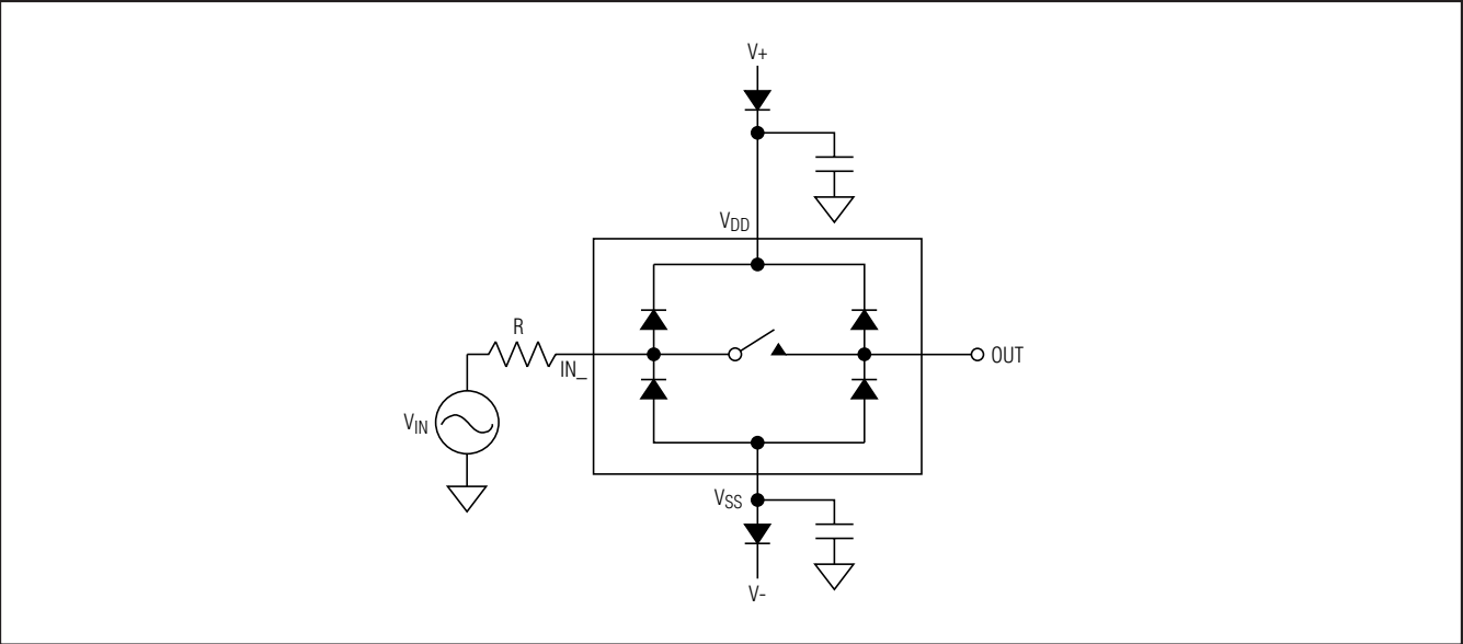
Figure 12. Beyond-the-Rail Application
