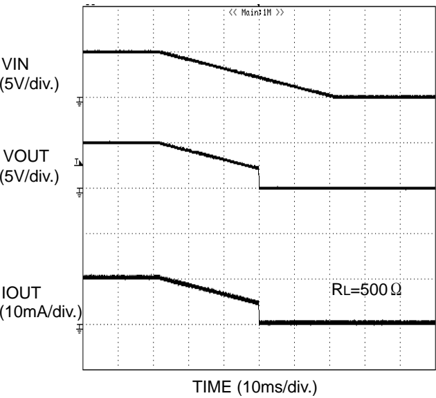
Figure 40. UVLO response decreasing VIN
