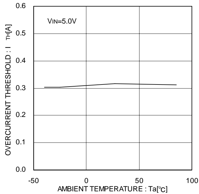
Figure 15. Over-current threshold
