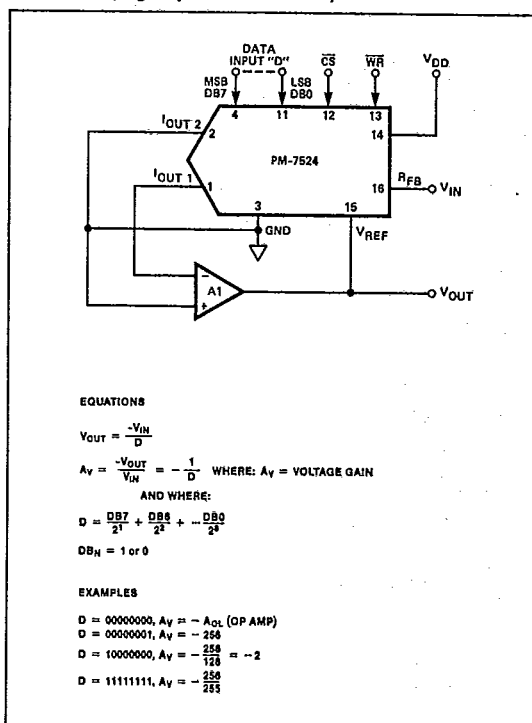
FIGURE 9: Divider (Digitally Controlled Gain)
