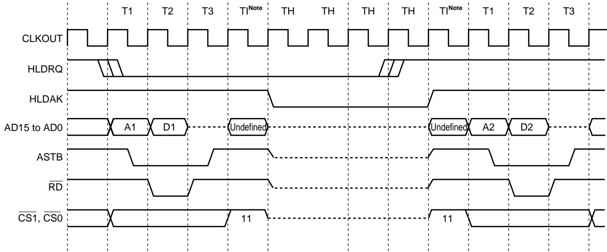
Figure 5-8. Bus Hold Timing (Bus Size: 16 Bits, 16-Bit Access)
