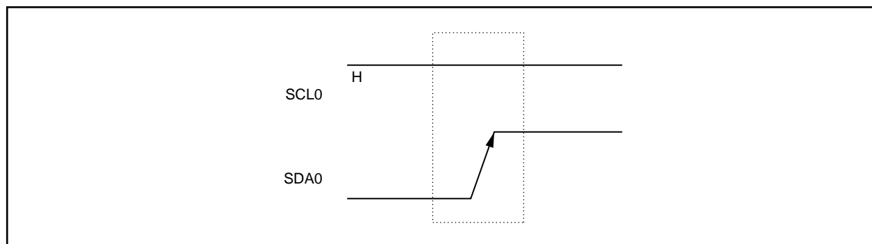
Figure 18-9. Stop Condition
