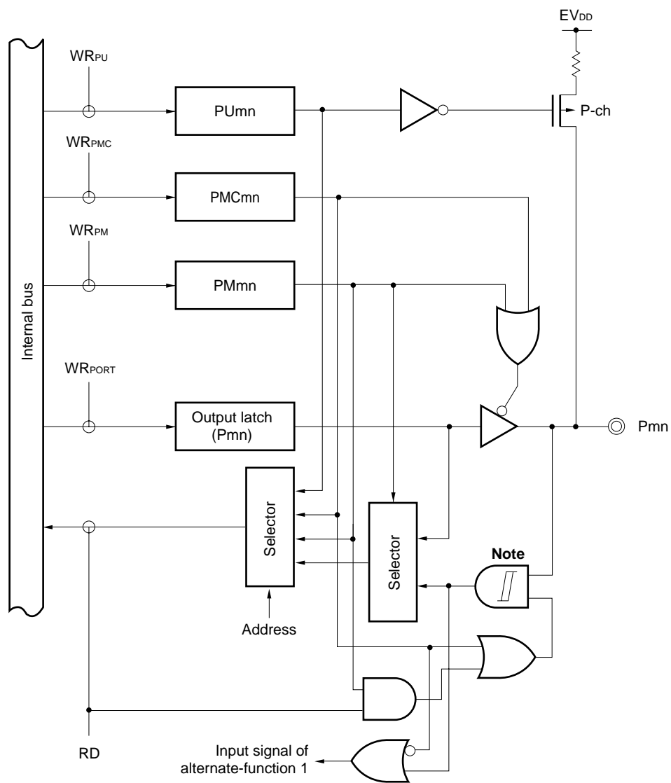
Figure 4-7. Block Diagram of Type D-1-1
