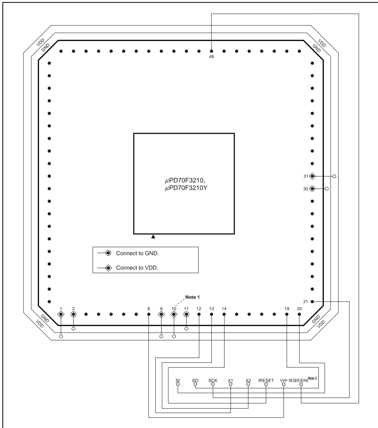
Figure 26-1. Wiring Example of V850ES/KF1 Flash Writing Adapter (FA-80GC-8BT, FA-80GK-9EU) (1/2)
