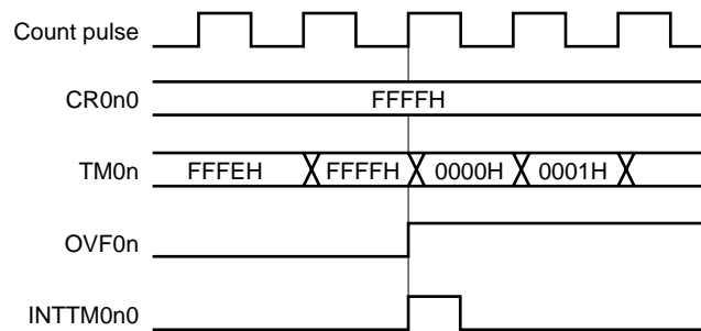
Figure 8-27. Operation Timing of OVF0n Flag
