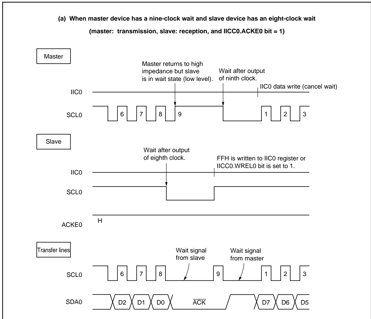
Figure 18-10. Wait Signal (1/2)
