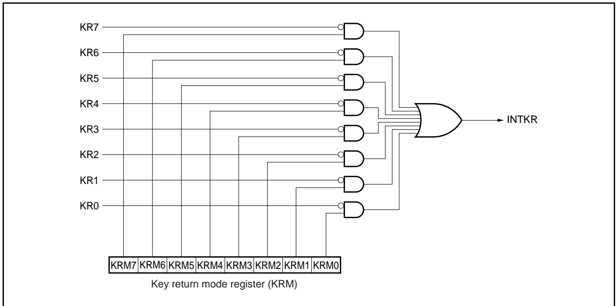
Figure 20-1. Key Return Block Diagram
