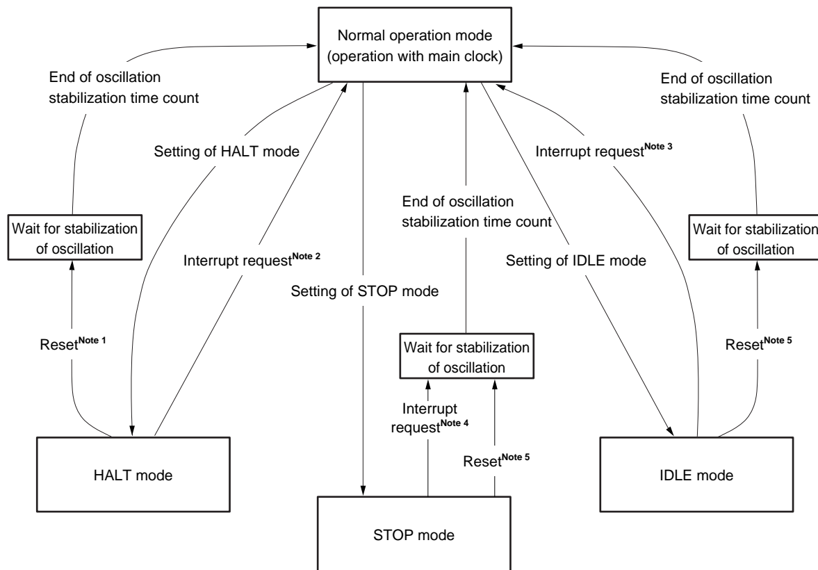
Figure 21-1. Status Transition (1/2)
