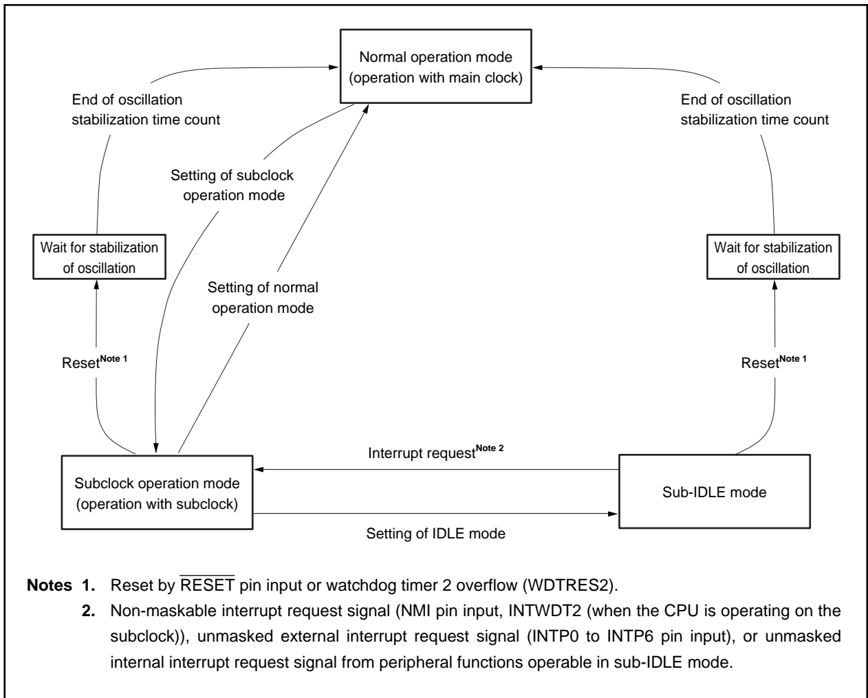
Figure 21-1. Status Transition (2/2)
