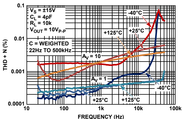
FIGURE 32. THD+N vs FREQUENCY vs TEMPERATURE, A_V = 1, 10, R_L = 10k
