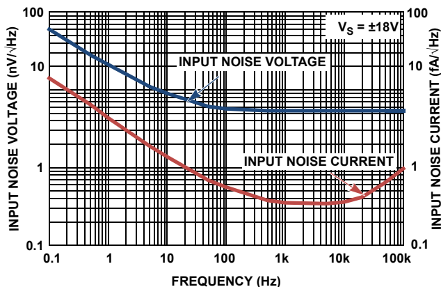
FIGURE 27. INPUT NOISE VOLTAGE (en) AND INPUT NOISE CURRENT (in) vs FREQUENCY, V_S = \pm 18V
