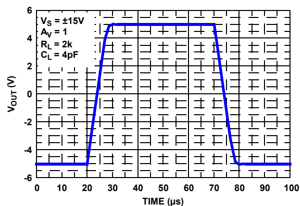
FIGURE 63. SIMULATED LARGE-SIGNAL 10V STEP RESPONSE
