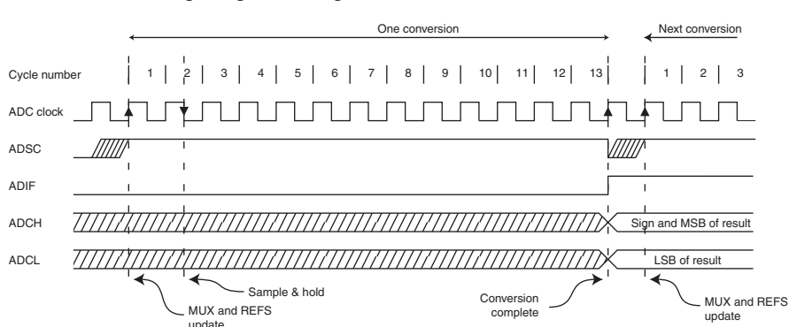
Figure 26-5. ADC timing diagram, single conversion.
