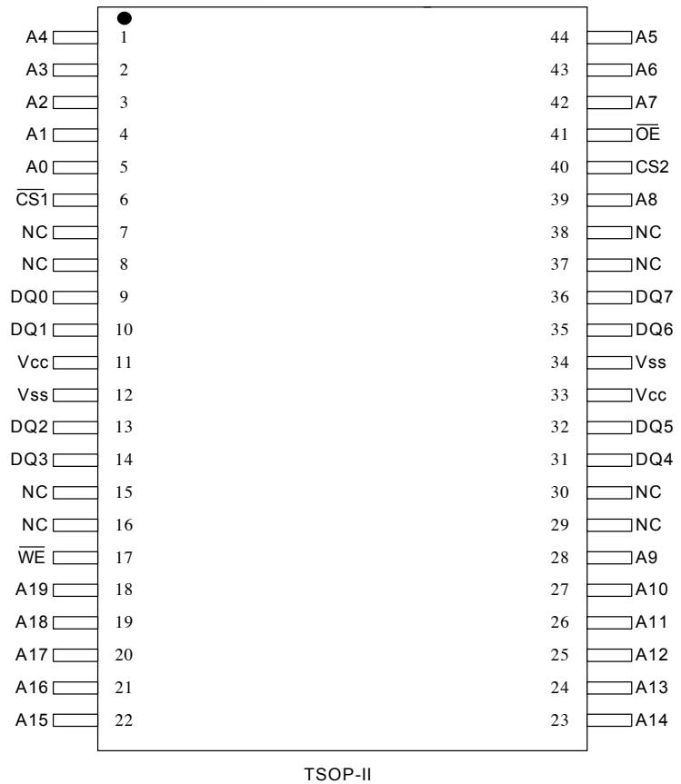
44 - TSOPII:Top view
