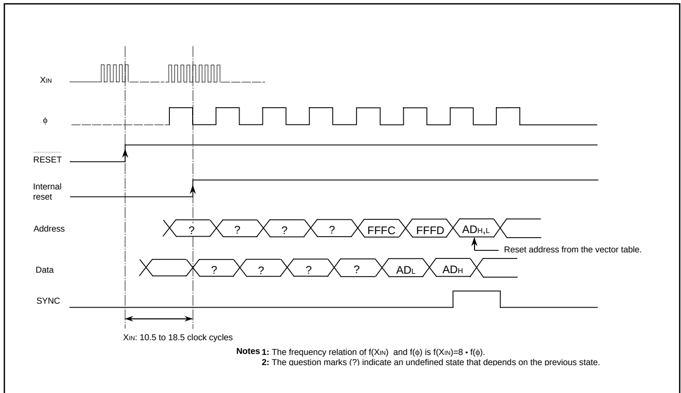
Fig. 79 Reset sequence
