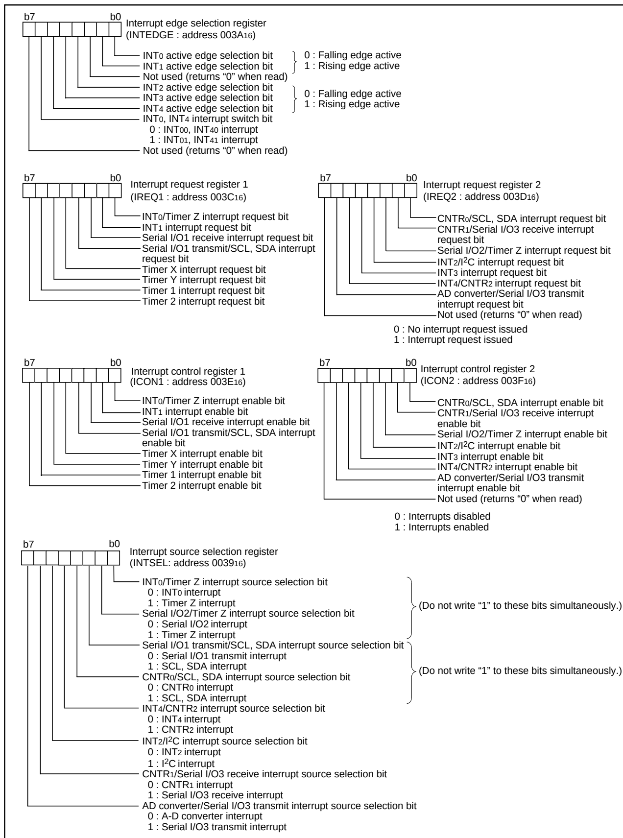
Fig. 28 Structure of interrupt-related registers of 3804 group
