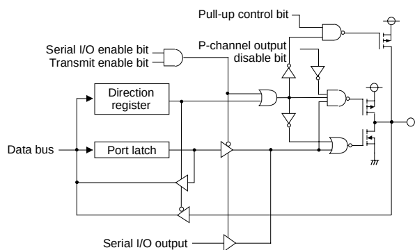
Fig. 19 Port block diagram of 3804 group (1)
