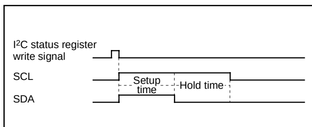
Fig. 70 START condition generating timing diagram
