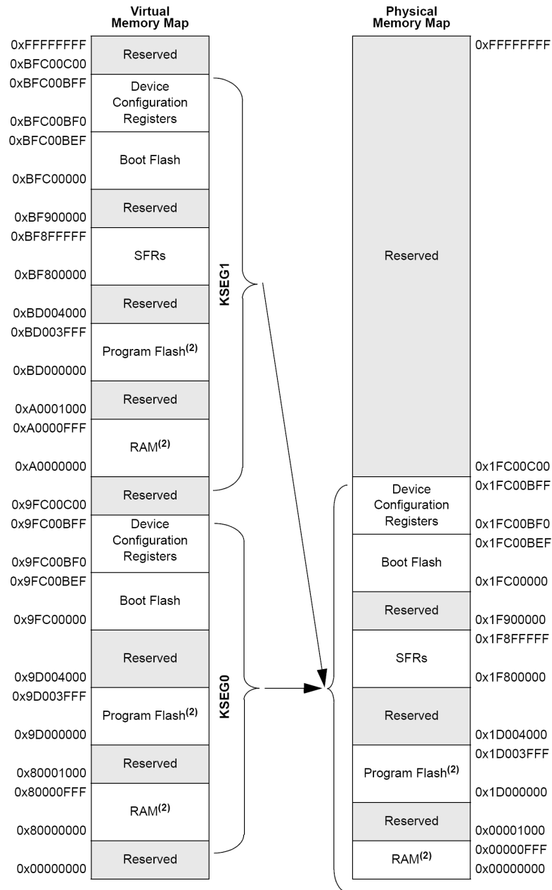
FIGURE 4-1: MEMORY MAP ON RESET FOR PIC32MX11X/21X DEVICES (1)
