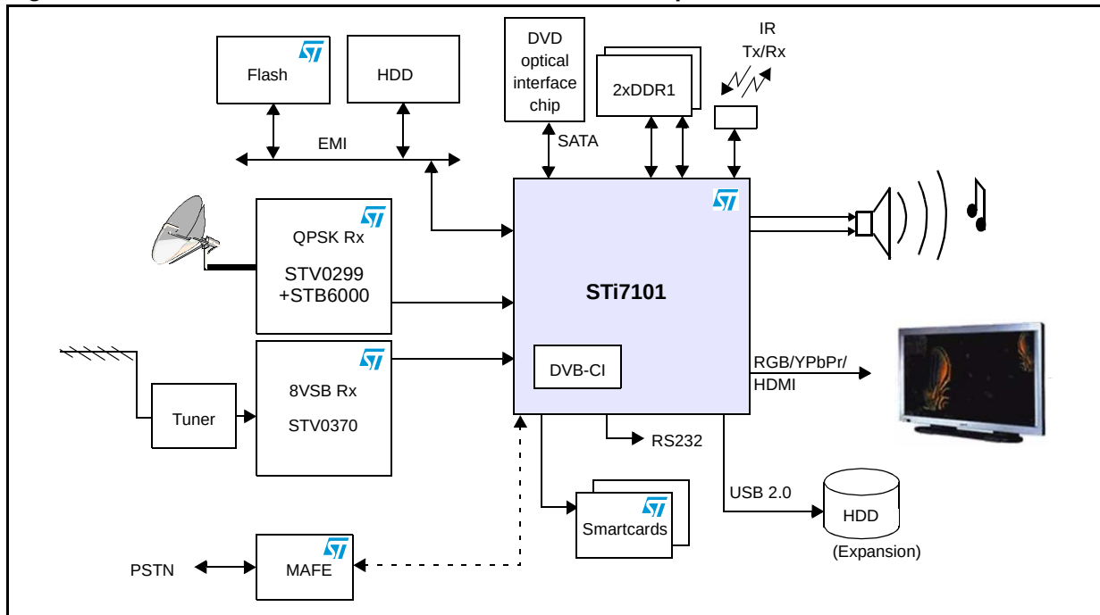
Figure 3. Low-cost dual satellite and terrestrial HD set-top box with HDD and DVD
