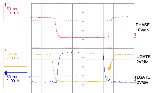
FIGURE 13. AC ADAPTER INSERTION
