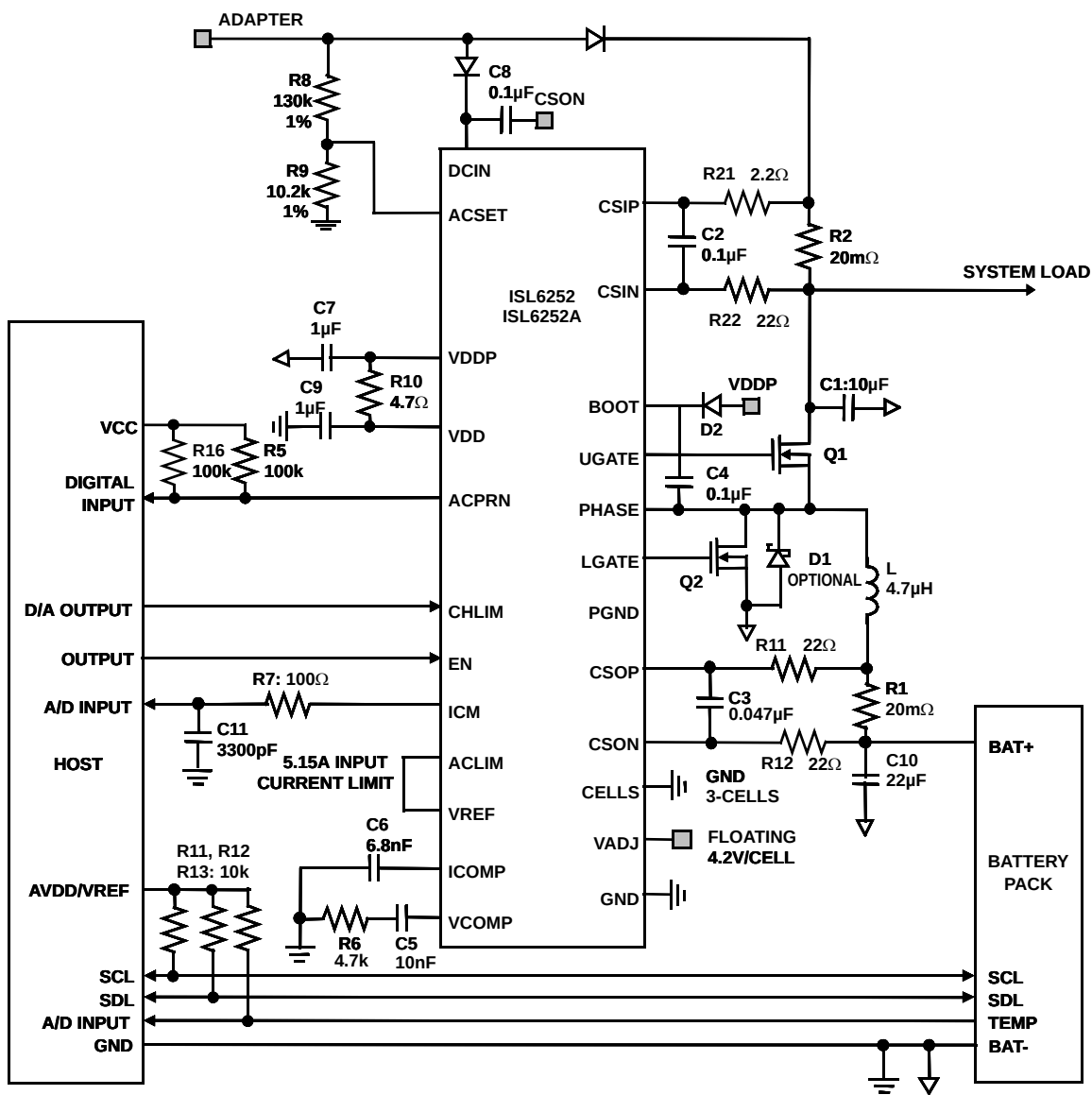
FIGURE 3. ISL6252, ISL6252A TYPICAL APPLICATION CIRCUIT WITH μP CONTROL
