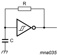
Fig. 12. Relaxation oscillator
