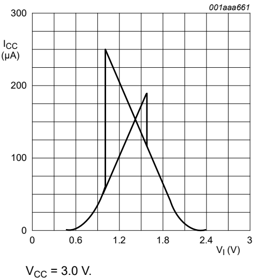
Fig. 10. Typical 74LV14 transfer characteristics
