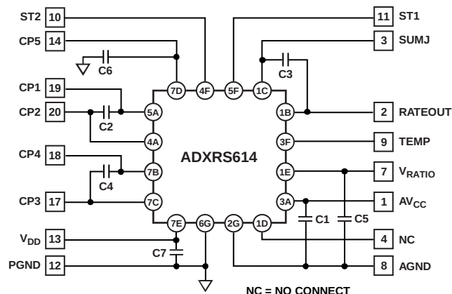
Figure 1. EVAL-ADXRS614 Schematic
