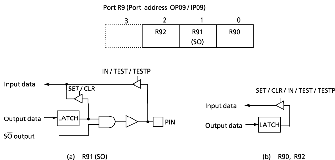
Figure 2-3. Port R9
