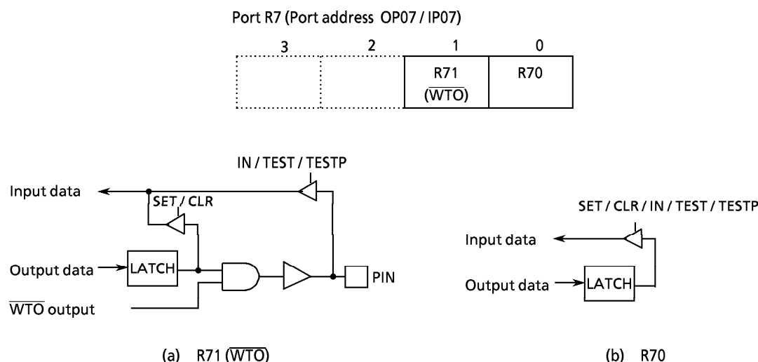
Figure 2-2. Port R7
