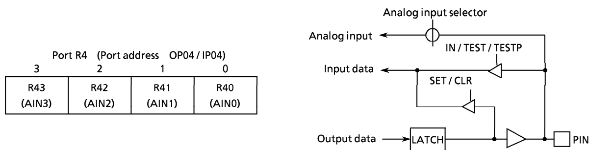
Figure 2-1. Port R4
