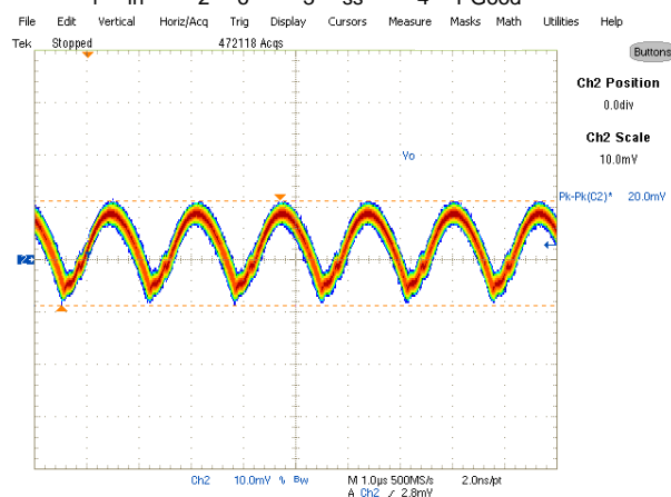
Fig. 10: Output Voltage Ripple, 12A load Ch 2 : V_{out}
