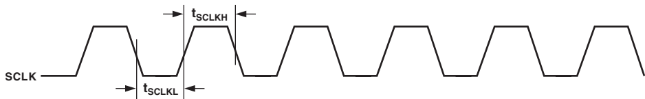
Figure 4. SCLK Switching Characteristics
