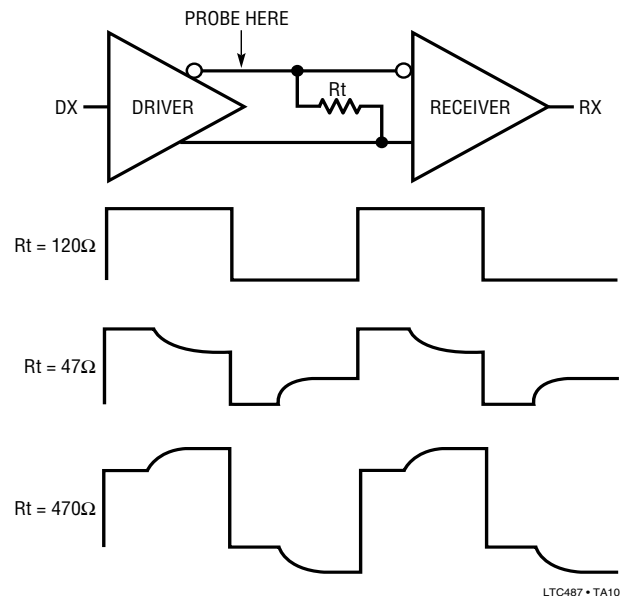
Figure 9. Termination Effects
